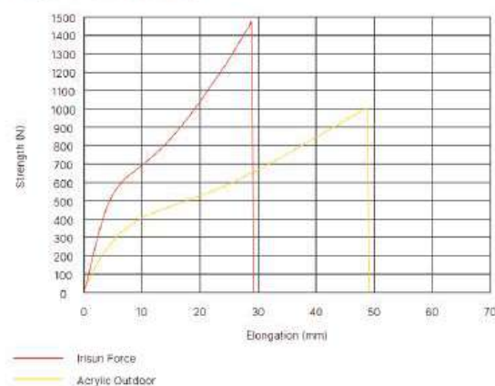
Elongation at break (ISO 13934-1): Weft Sample: 200 x 50 mm strip
